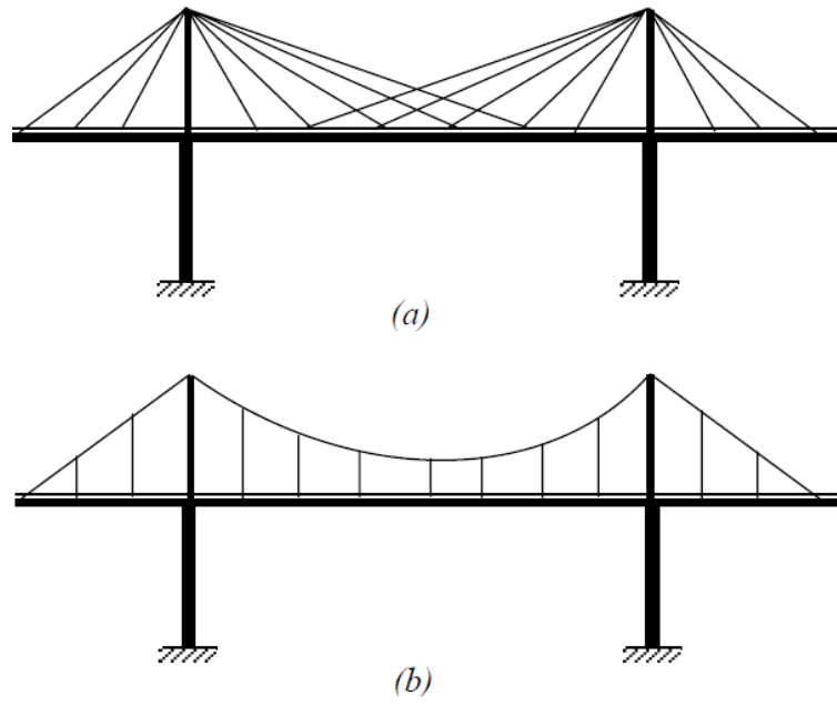
Figure 2.7 Cable-stayed structures
