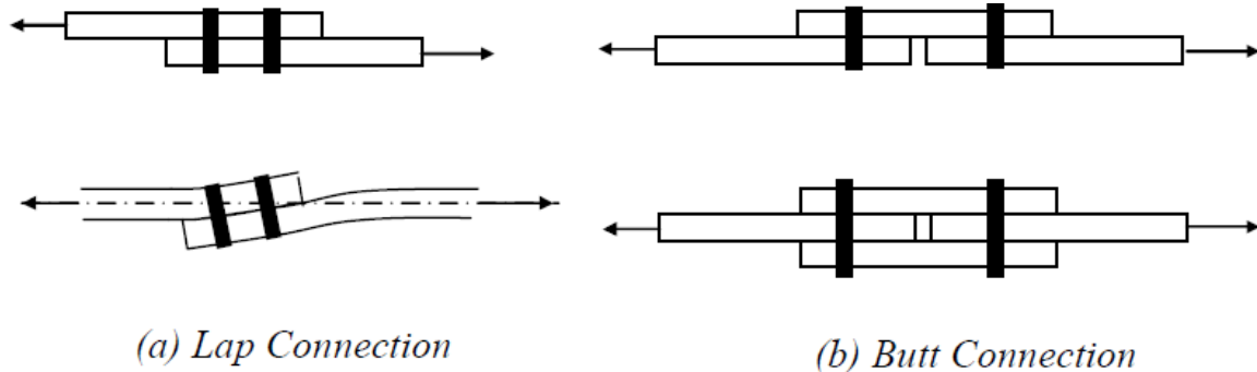
Figure 10.3 Shear connections
