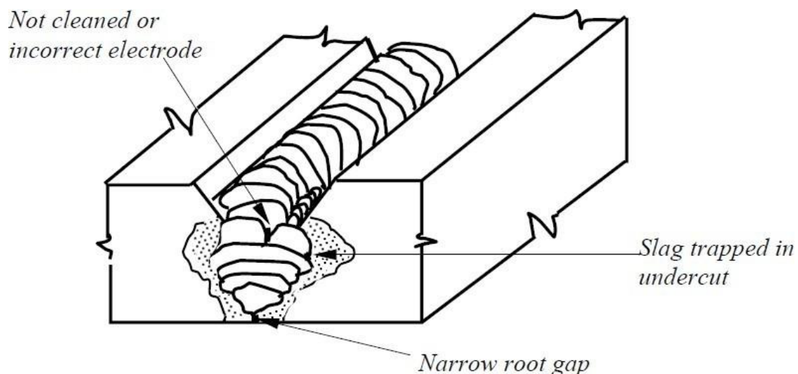
Figure 7.21 Slag inclusion
