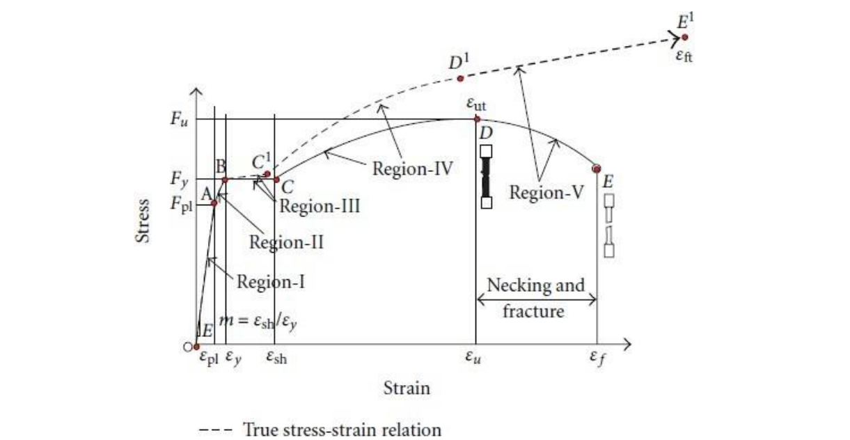
Figure 1.6 The engineering stress-strain relations and the proposed true stress-true strain material model
