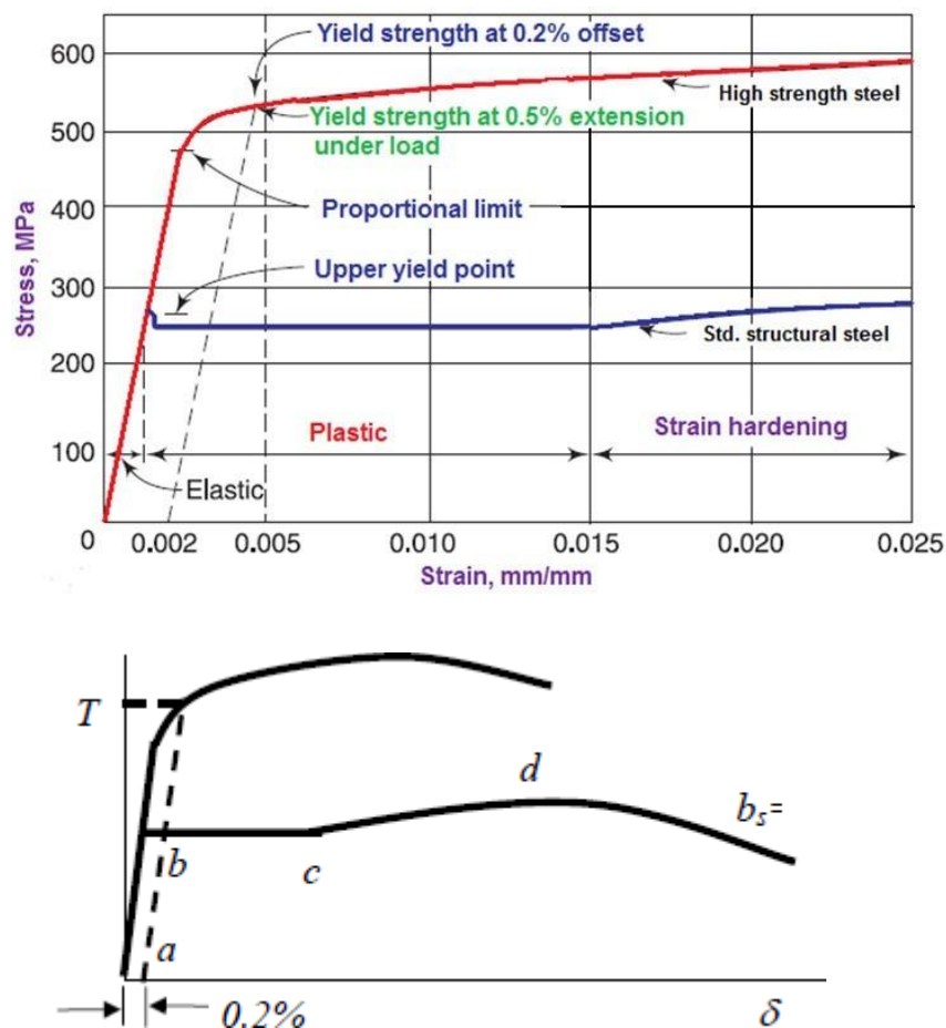
Figure 9.3 Load – Elongation of Tension Members
